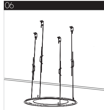
Hang the bracket to the rings
